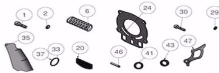
SPARE PARTS INCLUDED IN THE SERVICE KIT (The equipment includes grease and oil)
