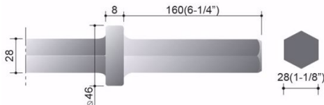
Shank: \varnothing 28 \times 160 mm
