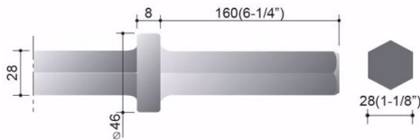
Shank: \varnothing 28x160mm
