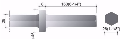
Shank: \varnothing 28 \times 160 \text{ mm}
